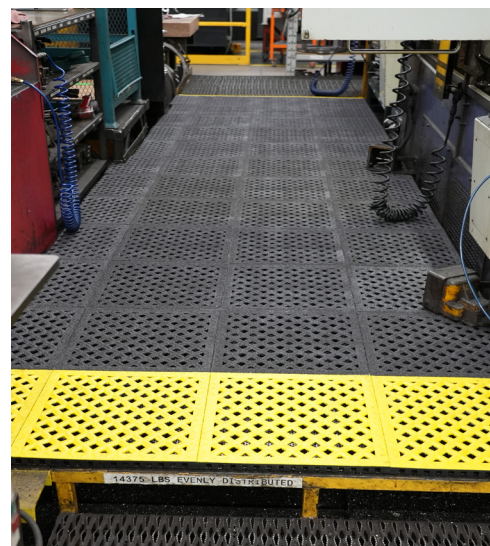
High Coolant Volume Areas Anti-Slip Drainage Tiles
